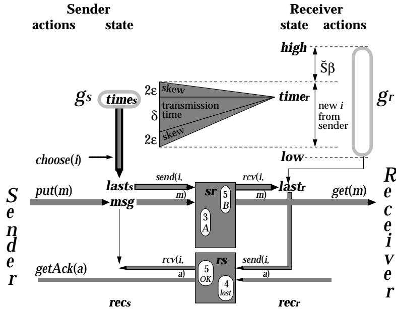
Figure 10.6. The flow of information in C
