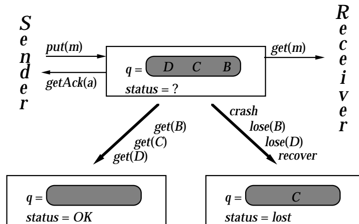
Figure 10.1. Some states and transitions for S
