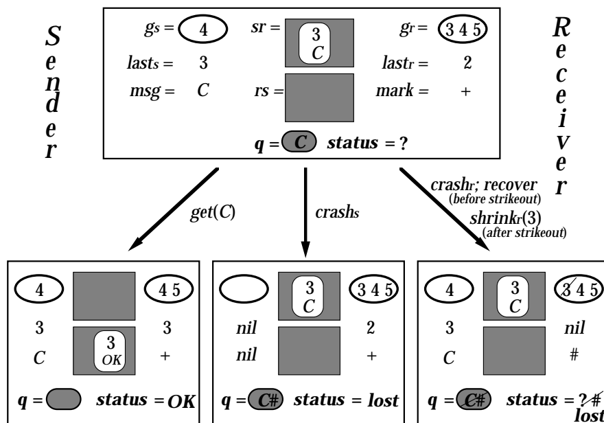
Figure 10.3. Some states and transitions of G
