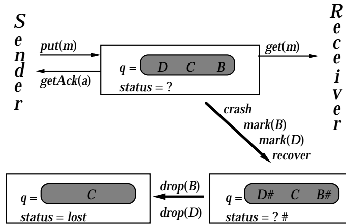
Figure 10.2. Some states and transitions of D
